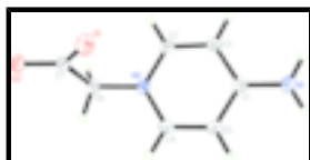
Fig. 1. The structure of 4-amino-pyridinium- N -acetate with the displacement ellipsoids shown at the 30% probability level.
